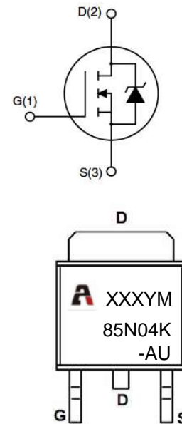
Marking and pin assignment
