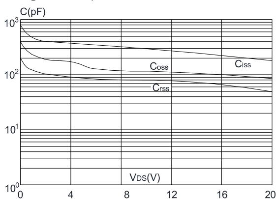
Figure 6: Capacitance Characteristics
