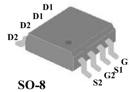
pin assignment
